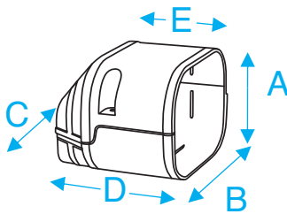
End Cover
