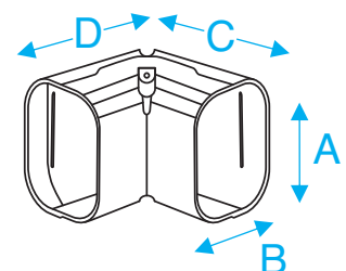
Flat Bend 90°
